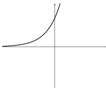
(e) y = e^x
