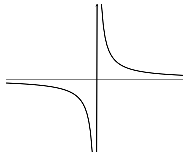
(c) y = \frac{1}{x}
