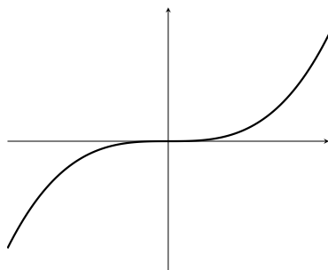
(a) y = x^3
